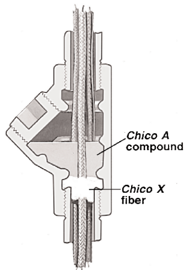
EYS 1 Vertical sealing
