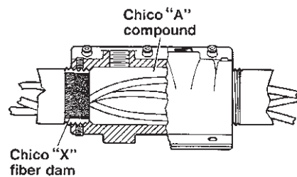
EYSR Retrofit seal
